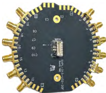
TF20-B-HTFD U4 Key B 20F fixture
