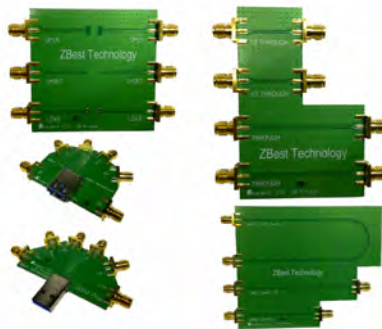
5R09T01 U3 Female fixture
